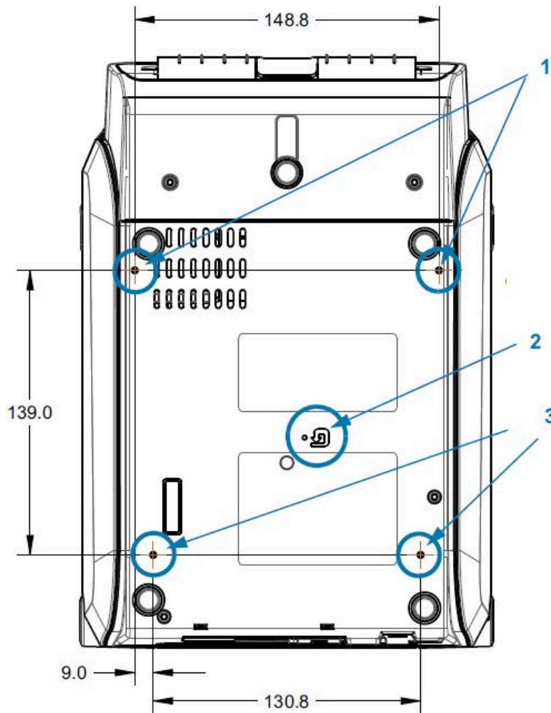
Figure 16 Mounting Specifications
