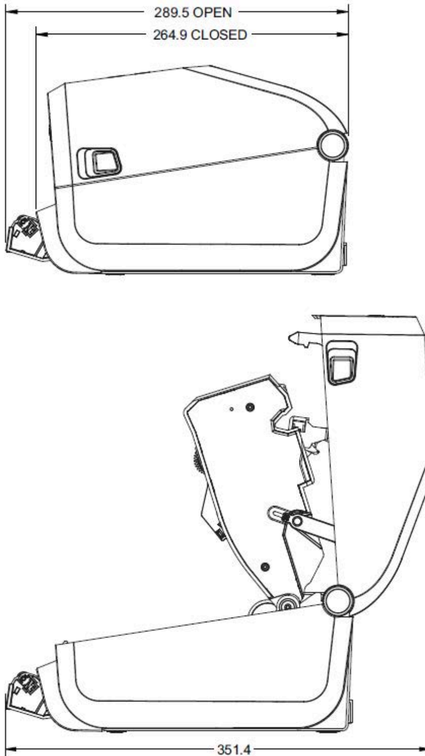
Figure 20 Ribbon Cartridge Thermal Transfer Printer with Label Dispenser (open)
